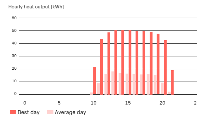
HOURLY HEAT OUTPUT OVER A DAY
