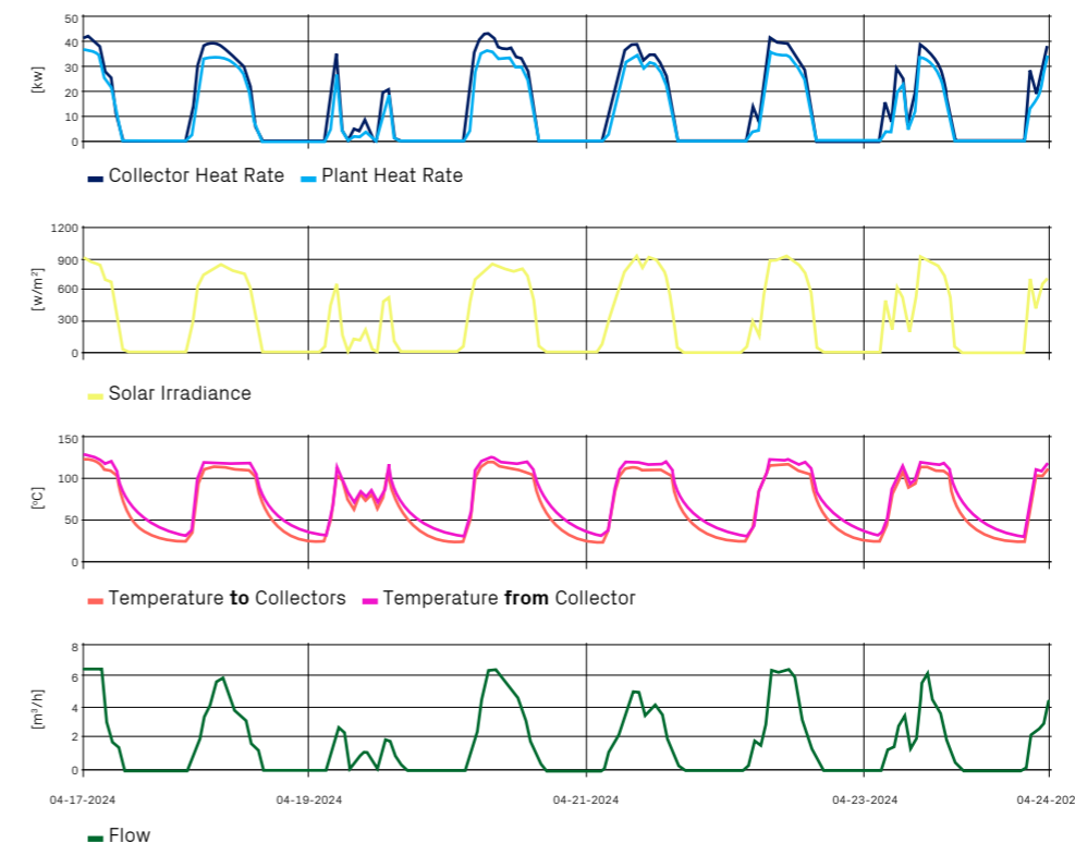
SYSTEM OPERATION OVER SEVERAL DAYS IN APRIL 2024
