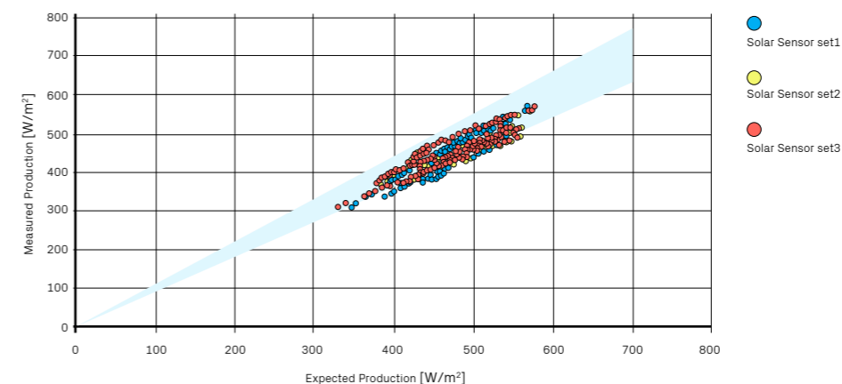
SOLAR FIELD POWER PERFORMANCE
